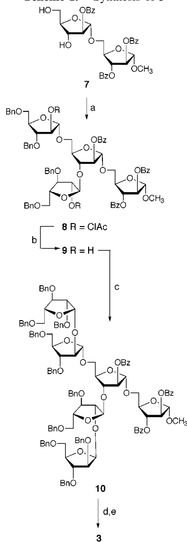
Scheme 1. Synthesis of 3 a
