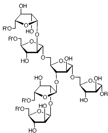
1 AG, R = arabinogalactan; R' = H or mycolic acids 2 LAM, R = arabinomannan; R' = H or Manp oligosaccharides 3 R = CH 3 ; R' = H
